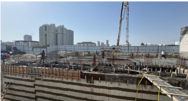
SLAB REINFORCEMENT
